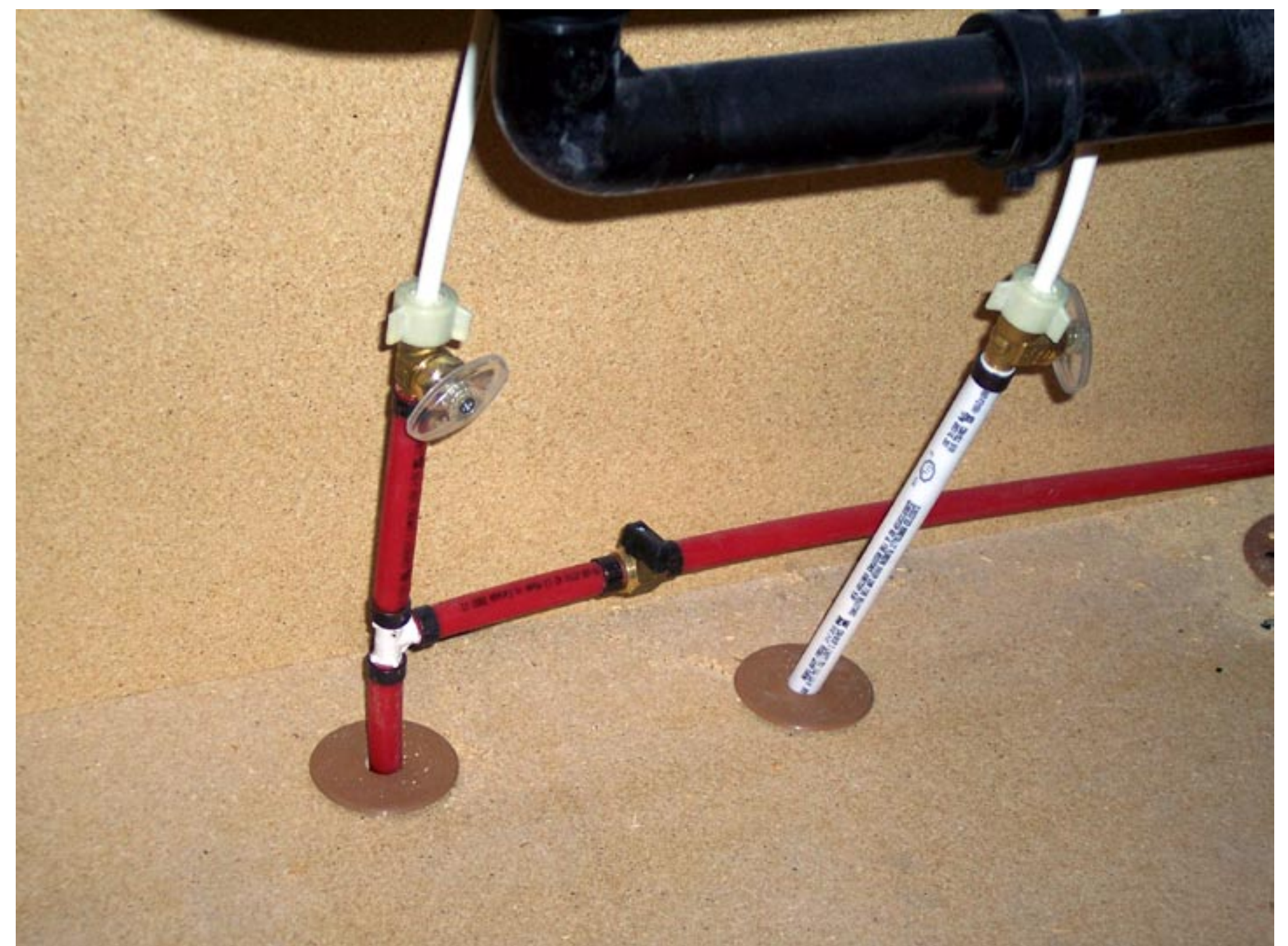
Organized and Clean Installation of Pex Hot and Cold Water Lines, Finished with Pipe Cover in Base Cabinets
